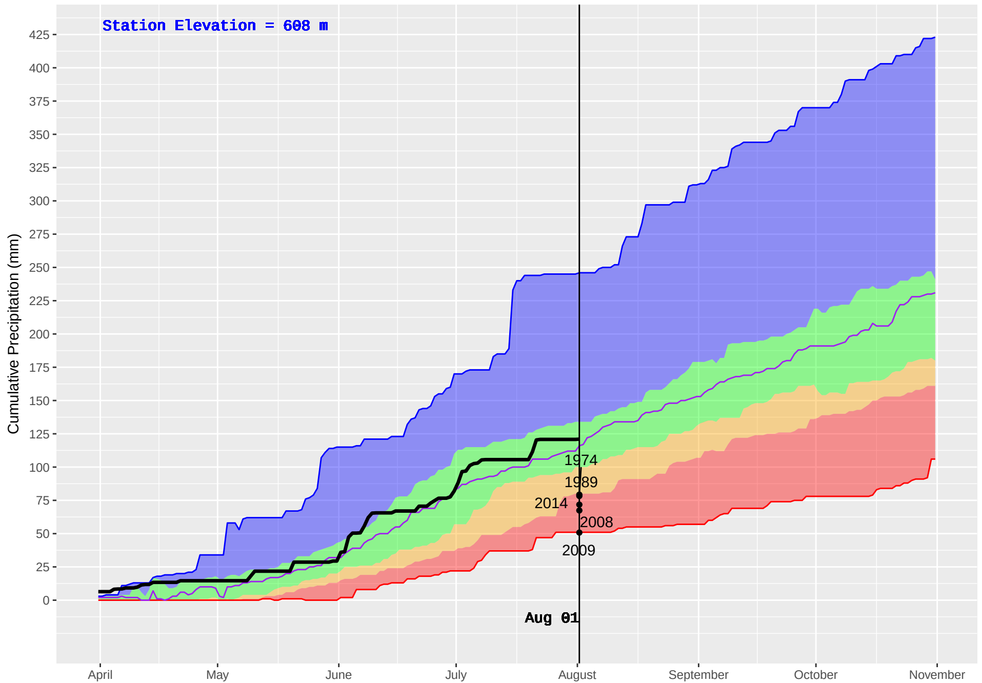
HOUSTON(DUNGATE) (162) : Historical (1974–2016) and Current (2018) Daily Cumulative Precipitation
