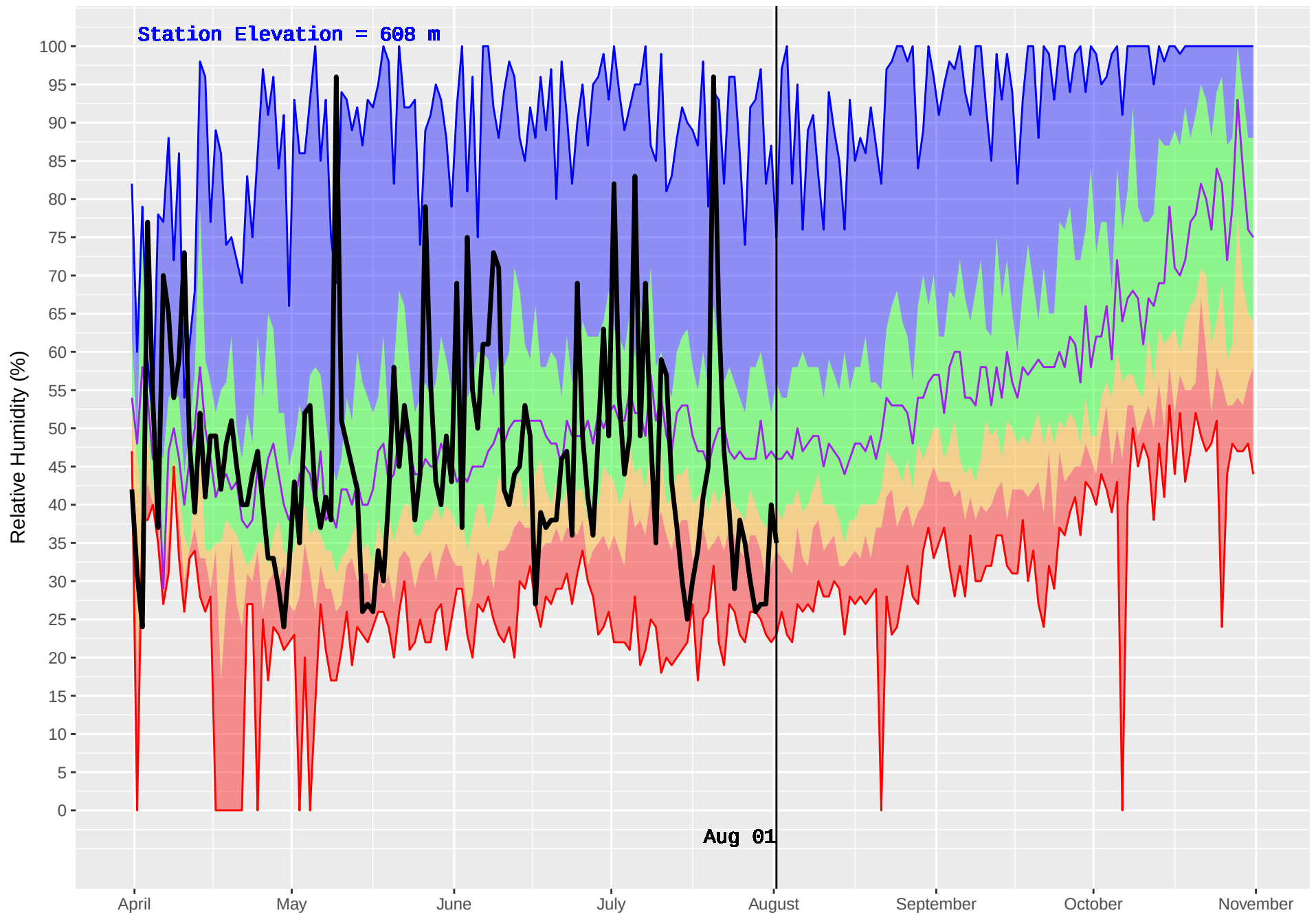
HOUSTON(DUNGATE) (162) : Historical (1974–2016) and Current (2018) Daily Relative Humidity
